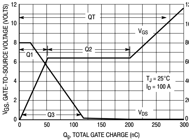
Figure 8. Gate Charge versus Gate-to-Source Voltage
